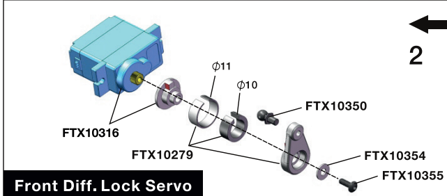
Diff.Lock (Front/Rear)
