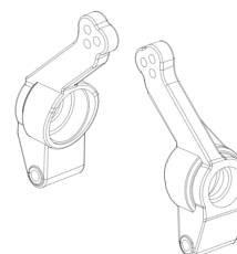
FTX10096 Aluminim rear hubs
